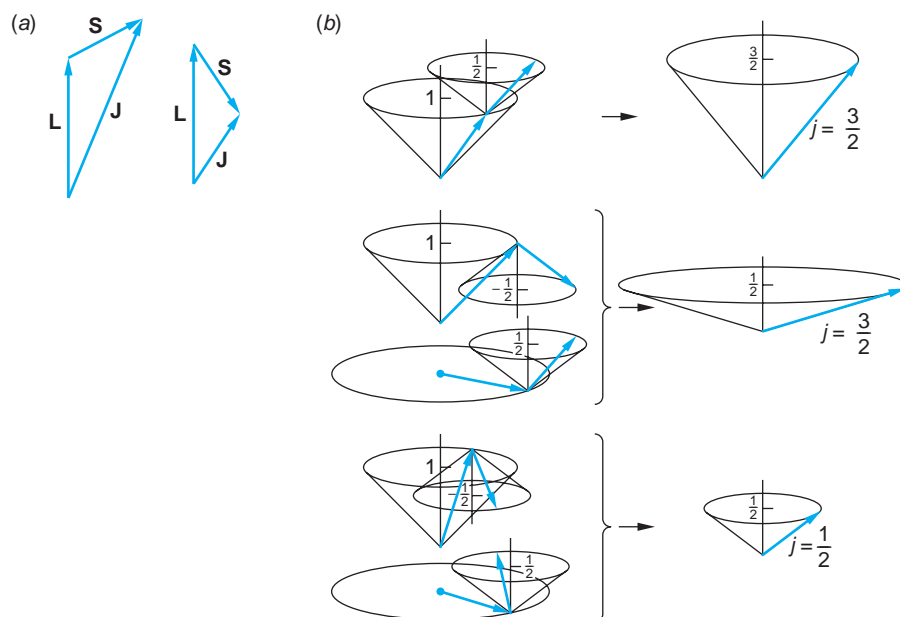
FIGURE 7-16 (a) Simplified vector model illustrating the addition of orbital and spin angular momenta. Case shown is for \ell = 1 and s = \frac{1}{2} . There are two possible values of the quantum number for the total angular momentum: j = \ell + s = \frac{3}{2} and j = \ell - s = \frac{1}{2} . (b) Vector addition of the orbital and spin angular momenta, also for the case \ell = 1 and s = \frac{1}{2} . According to the uncertainty principle, the vectors can lie anywhere on the cones corresponding to the definite values of their z components. Note in the middle sketch that there are two ways of forming the states with j = \frac{3}{2} , m_j = \frac{1}{2} and j = \frac{1}{2} , m_j = \frac{1}{2} .
